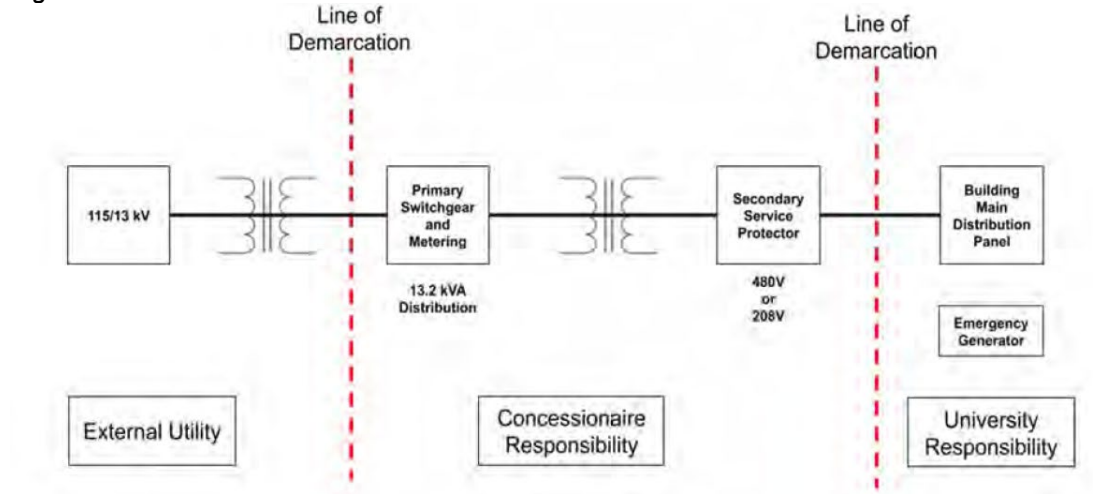
Figure 330100-3 – Electrical Demarcation
