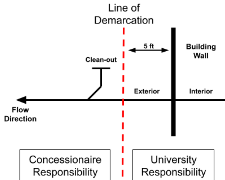
Figure 330100-8 – Sanitary Sewer Demarcation
