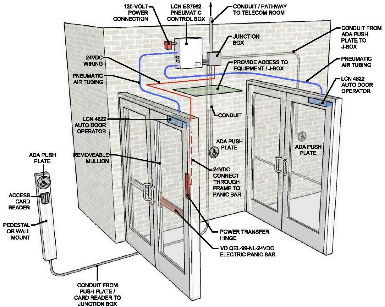
Figure 281000-1 – Example of Access Control Layout with ADA Operators and Card Reader
