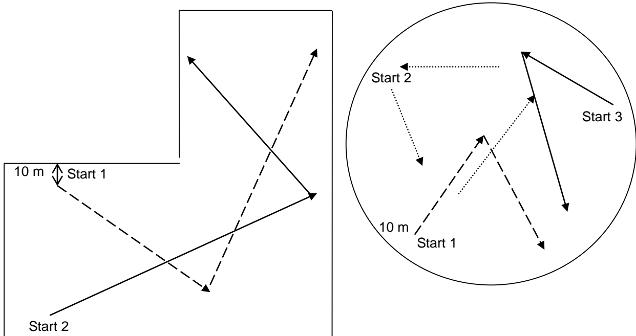
Figure 2. Sample patterns for inspecting circle- and irregular-shaped fields
