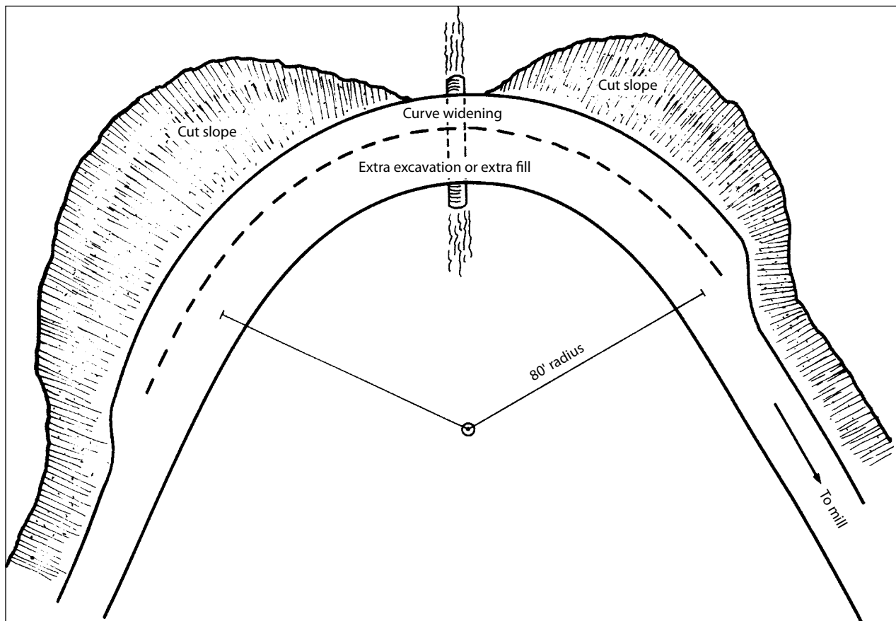
Figure 11. Curve widening to permit truck passage on sharp curves
