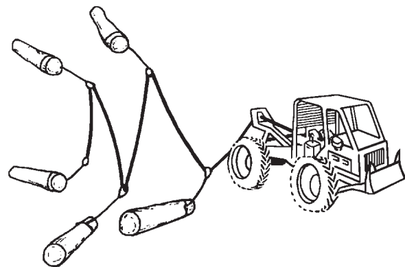
Figure 19 — Chokers may be attached to the winch line by sliding hooks. A ferrule at the end of the line keeps the chokers from sliding off.
