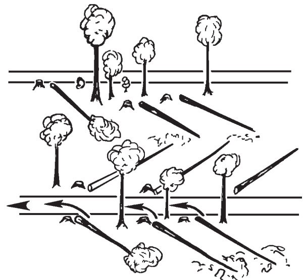
Figure 17 — Directional felling with the butts of the trees toward the skid trail. This method is recommended for larger trees.
